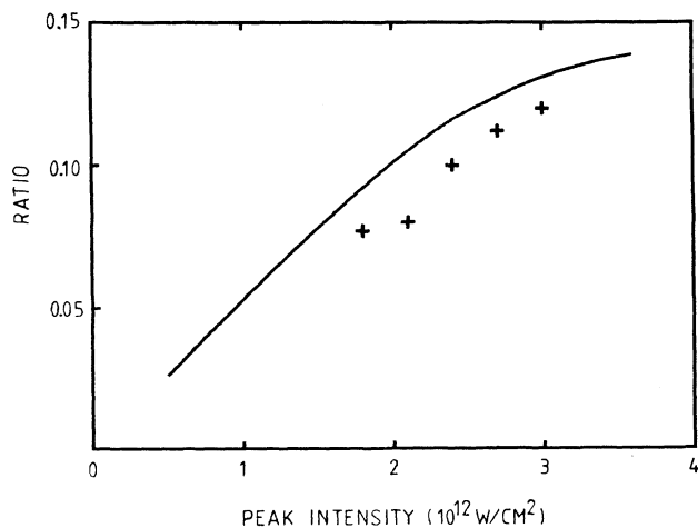
FIG. 3. Ratio between 4- and 5-photon detachments as a function of the peak intensity. Pluses: experimental results; continuous line: theoretical calculations [11].
