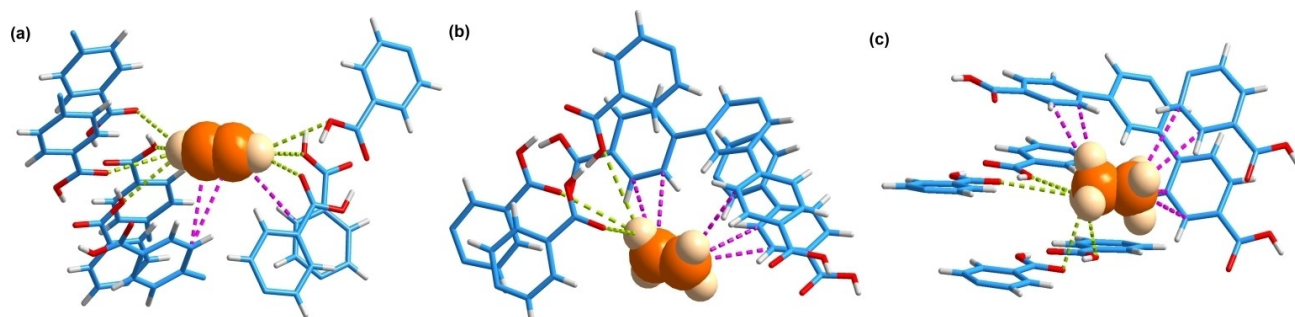
Figure 3. The calculated preferential adsorption sites for (a) C_2H_2 , (b) C_2H_4 and (c) C_2H_6 in HOF-TDCPB. The C-H\cdots O hydrogen bonds are shown in dashed green lines and the C-H\cdots\pi interactions between gas molecule and the pore surface are shown in dashed purple lines. For clarity, C_2H_2 , C_2H_4 and C_2H_6 molecules are in space-filling model.
