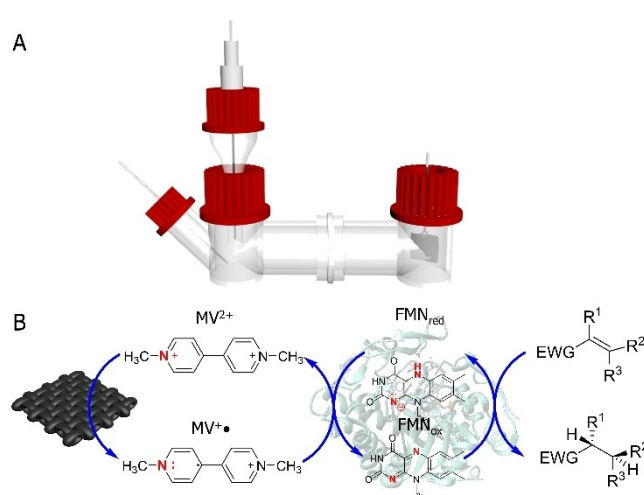
Scheme 2. The system using MV 2+ as a mediator molecule for bio-electrocatalytic reaction. (a) The design of the electrochemical cell. (b) Schematic of the bio-electrocatalytic process.
