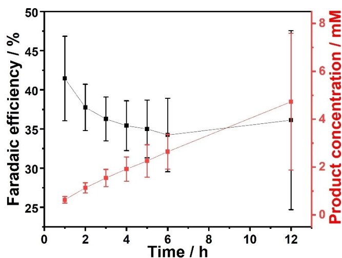
Figure 2. The concentration of cyclohexanone product obtained in the biocatalytic reduction of 2-cyclohexen-1-one (1) using the MV 2+ /MV •+ regeneration system and the faradaic efficiency of this system. The reaction solution contained 10 μM PETNR, 1 mM MV 2+ in 0.1 M pH = 7.4 KPi buffer with 0.1 M KCl. The concentration of 1 was 10 mM. Error bars represent the standard deviation of three independent experiments.
