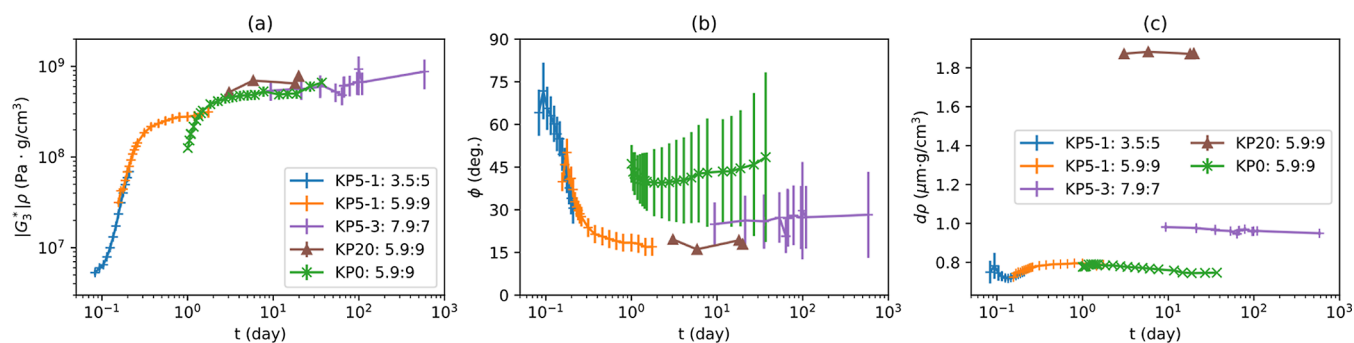
Figure 4. Evolution of |G_3^*|\rho (a), \phi (b), and \Delta\rho (c) for the KP films with no added PbO (KP0), with 5 wt % PbO (KP5–1 and KP5–3) and 20 wt % PbO (KP20). The legend for (b) is identical to the legends for (a,c).
