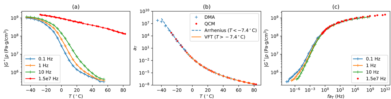
Figure 5. (a) Temperature dependence of |G_3^*|\rho at 1.5 \times 10^7 Hz from the QCM data and at much lower frequencies from the DMA data from Baij et al. 48 (b) Temperature-dependent shift factors with an Arrhenius fit (eq 6, E_a = 300 kJ/mol) for temperatures less than -7.4 °C and a Vogel–Fulcher–Tammann fit (eqs 7) for temperatures above -7.4 °C. (c) Master curve for |G_3^*|\rho using the temperature shift factors from part (b).
