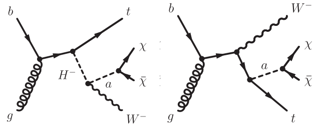
Fig. 3. Representative Feynman diagrams for the dominant production modes for the E_T^{\text{miss}} + tW signature in the 2HDM+a.
