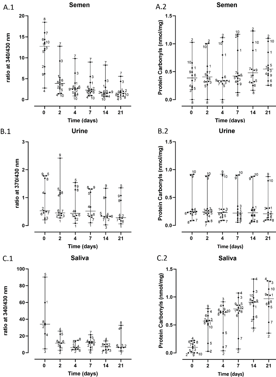
Figure S1: Distribution of the fluorescent ratios (.1) and the protein carbonyls concentrations (.2) of each donor for semen, urine and saliva. The whiskers indicate the range from the smallest to the largest value.
