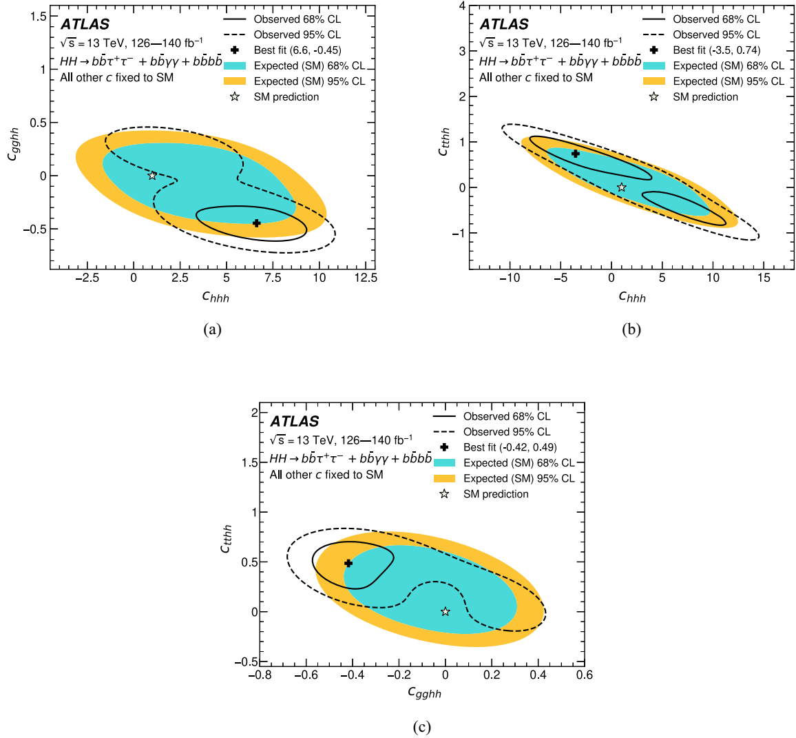
FIG. 4. Two-dimensional test-statistic contours at 68% CL (solid line) and 95% CL (dashed line) in the (a) c_{gggh} - c_{hhh} , (b) c_{tthh} - c_{hhh} , and (c) c_{tthh} - c_{gggh} HEFT parameter spaces, with c_{tthh} , c_{gggh} , and c_{hhh} fixed to their SM values, respectively. The corresponding SM expected contours are shown by the inner and outer shaded regions. The SM prediction is indicated by the star, while the best-fit value is shown by the cross.
