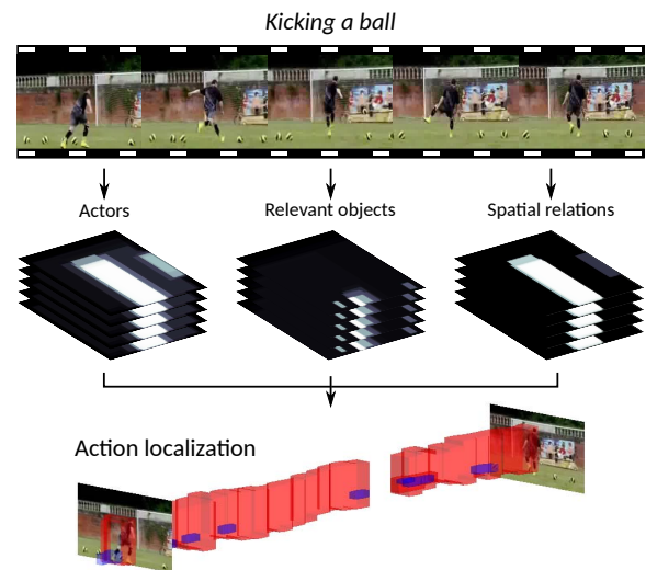
Figure 1: Spatial-aware object embedding. Actions are localized and classified by information about actors, relevant objects, and their spatial relations.
