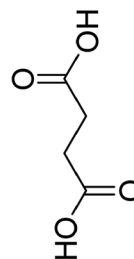
succinic acid
