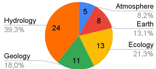
Fig. 2. Earth science domains
