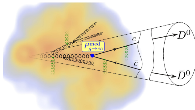
FIG. 1. Illustration of a parton shower containing a g \rightarrow c\bar{c} splitting. This c\bar{c} radiation is enhanced due to the QGP, which can be tested by measuring D^0\bar{D}^0 pairs inside jets.
