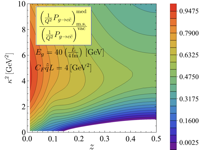
FIG. 2. The ratio of medium modification over vacuum splitting P_{g \rightarrow c\bar{c}}^{\text{med}}/P_{g \rightarrow c\bar{c}}^{\text{vac}} \equiv P_{g \rightarrow c\bar{c}}^{\text{tot}}/P_{g \rightarrow c\bar{c}}^{\text{vac}} - 1 shows an enhancement of nearly 100% over the vacuum baseline in a significant phase space region [see Eq. (5)].
