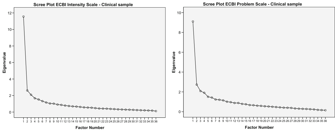
Fig. 2 Scree plots ECBI Intensity and Problem Scale for clinical sample
