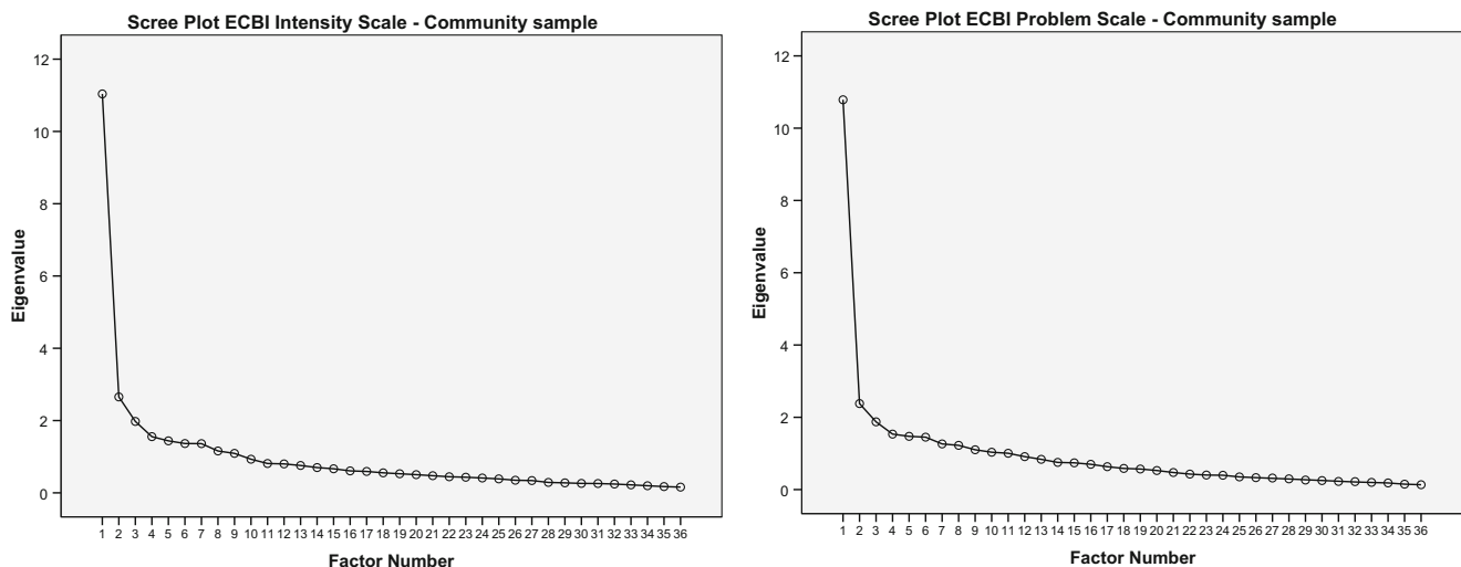
Fig. 1 Scree plots ECBI Intensity and Problem Scale for community sample
