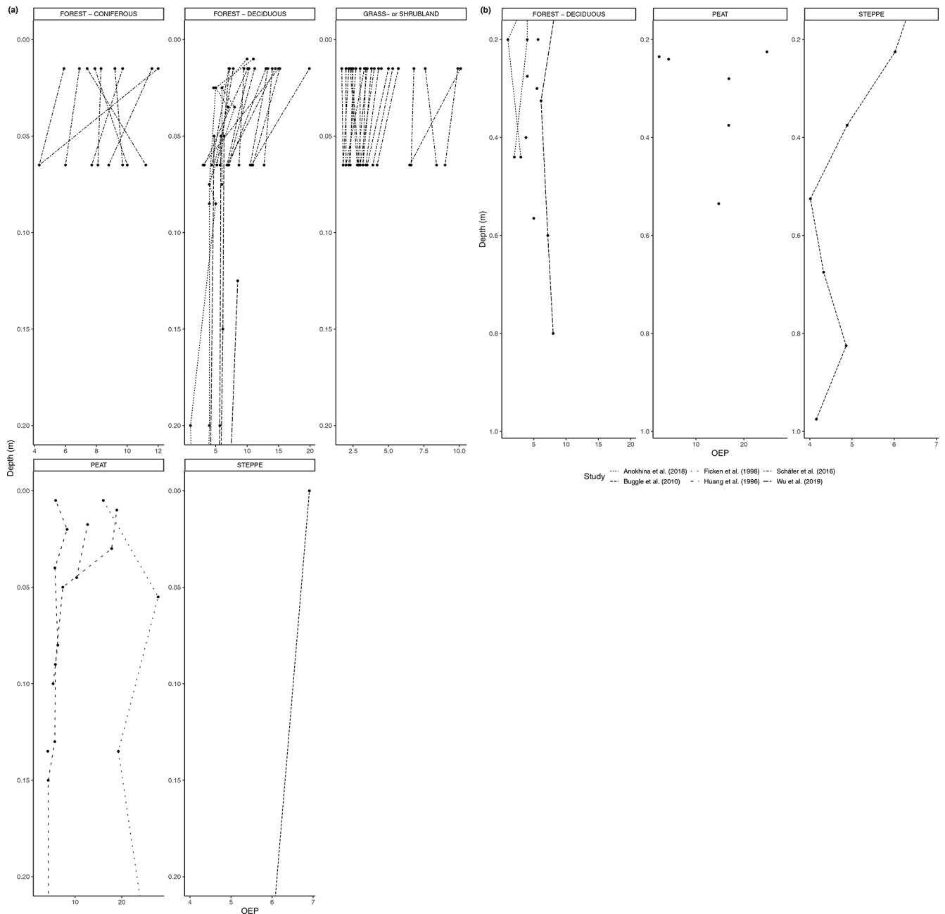
Figure 9. (a) OEP of n -alkanes in soil from 0 to 20 cm. (b) OEP of n -alkanes in soil below 20 cm.
