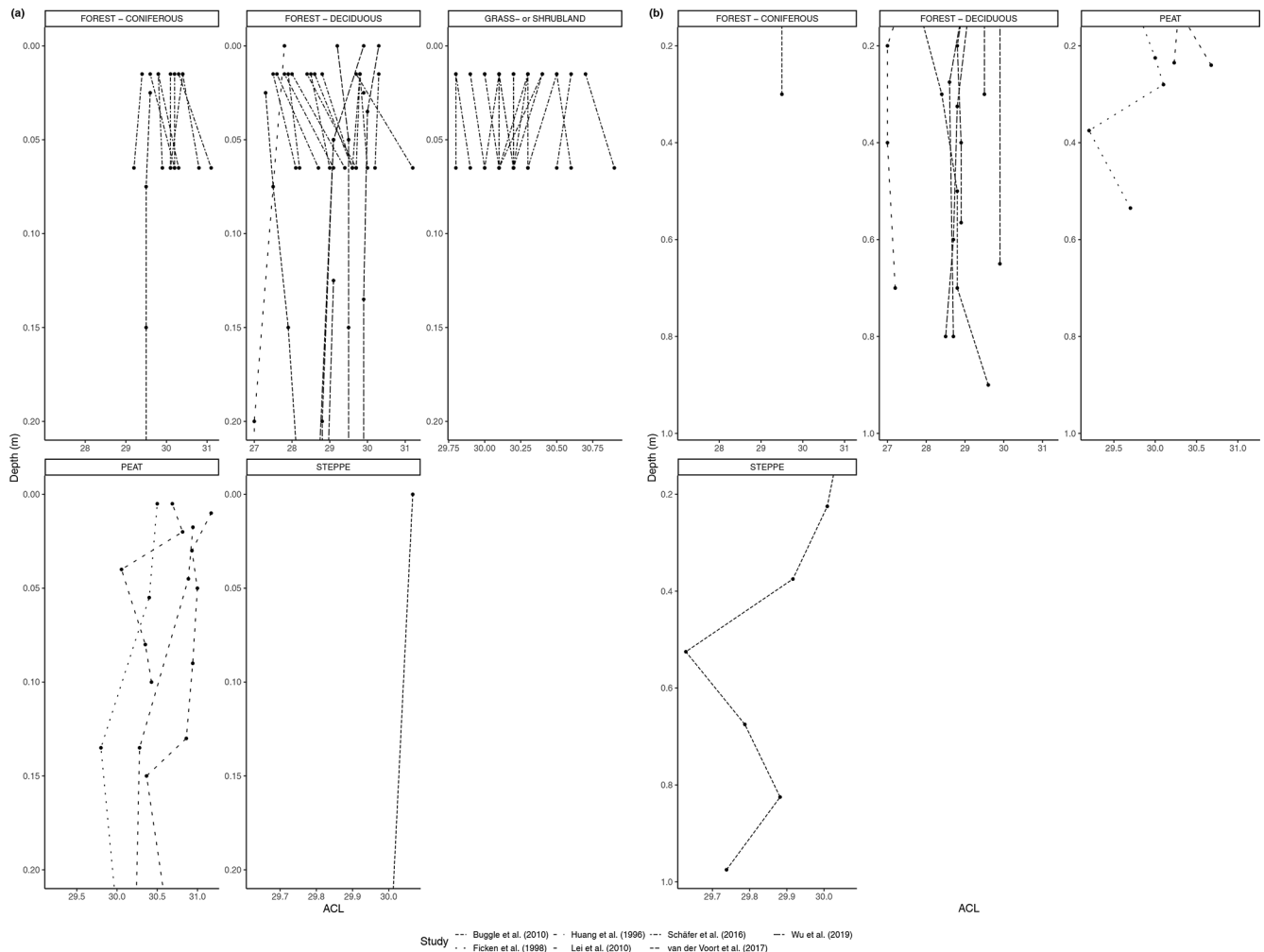
Figure 7. (a) ACL of n -alkanes in soil from 0 to 20 cm. (b) ACL of n -alkanes in soil below 20 cm.
