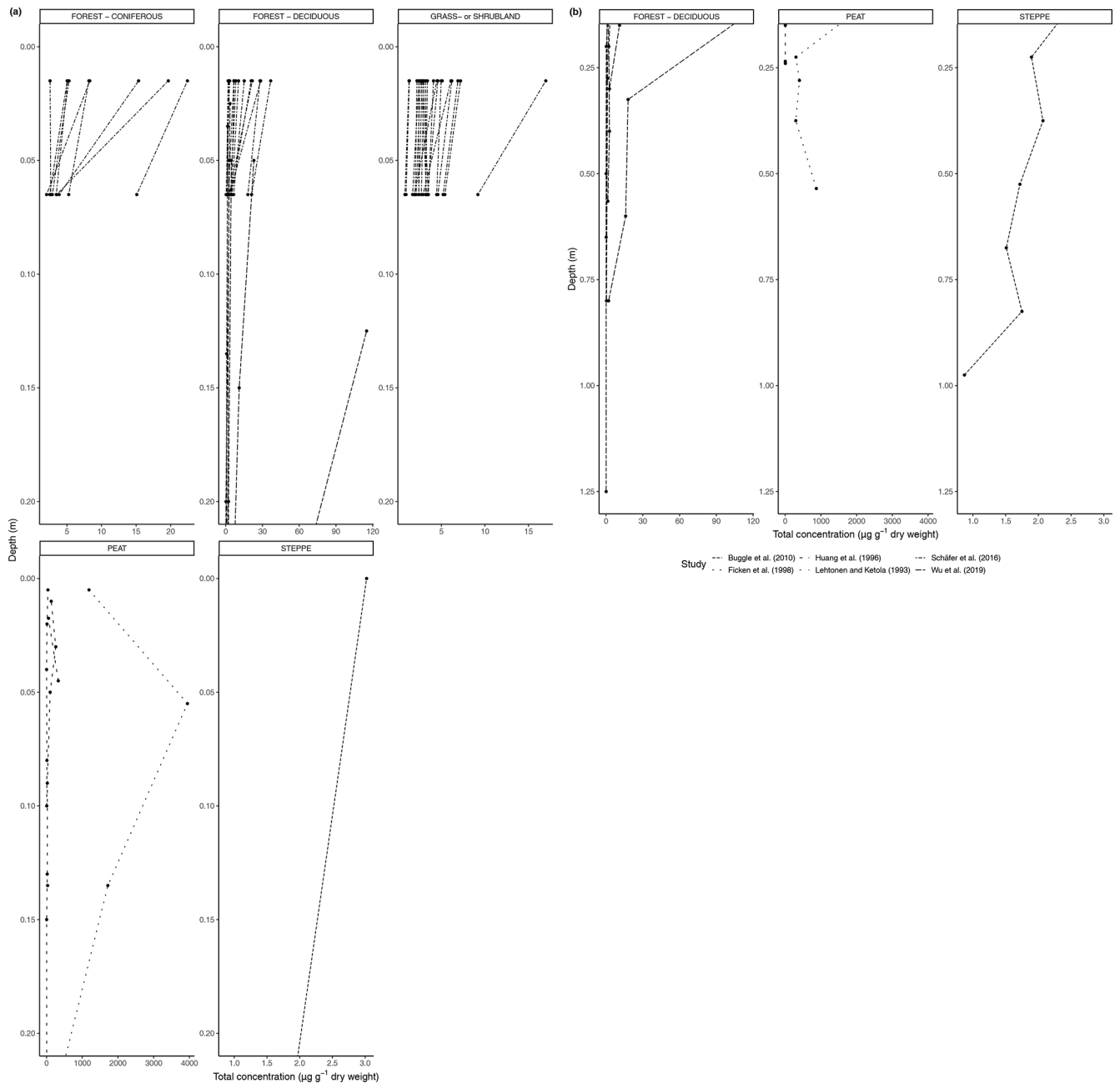
Figure 5. (a) Total concentration ( \mu\text{g/g} dry weight) of n -alkanes in soil from 0 to 20 cm. (b) Total concentration ( \mu\text{g/g} dry weight) of n -alkanes in soil below 20 cm.
