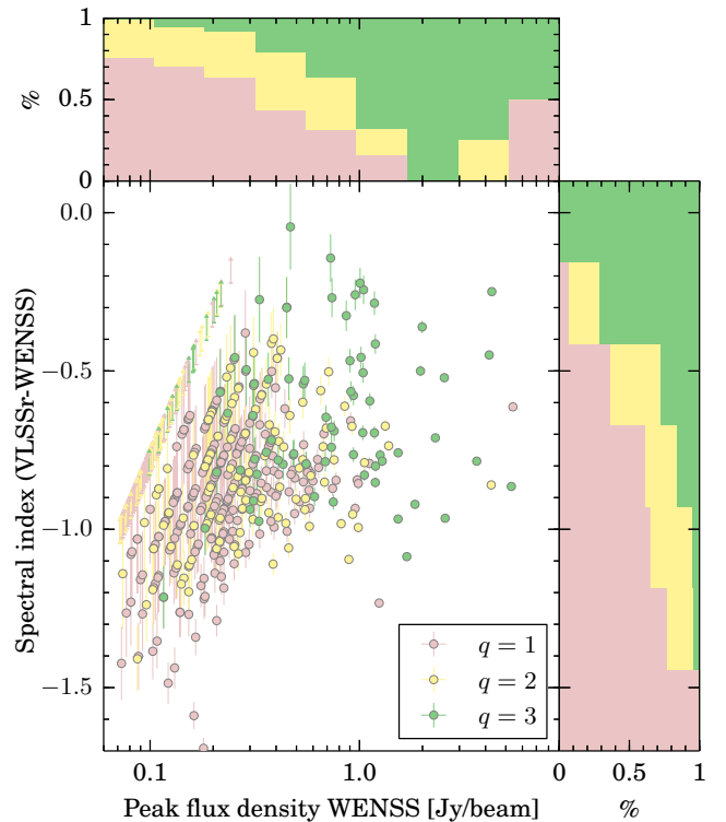
Fig. 7. Source quality as a function of low-frequency spectral index and WENSS peak flux density. Red, yellow, and green colours represent q = 1, 2, and 3 , respectively. q = 3 corresponds to suitable primary calibrators. The histograms show the percentage of sources at each quality value. The histogram on the right does not include the sources with upper limits in their spectral indexes. The uncertainties of some of the values are smaller than the symbols, especially for the WENSS peak flux density. The stripes at low peak flux densities are due to sources detected at multiples of the rms noise of VLSSr.
