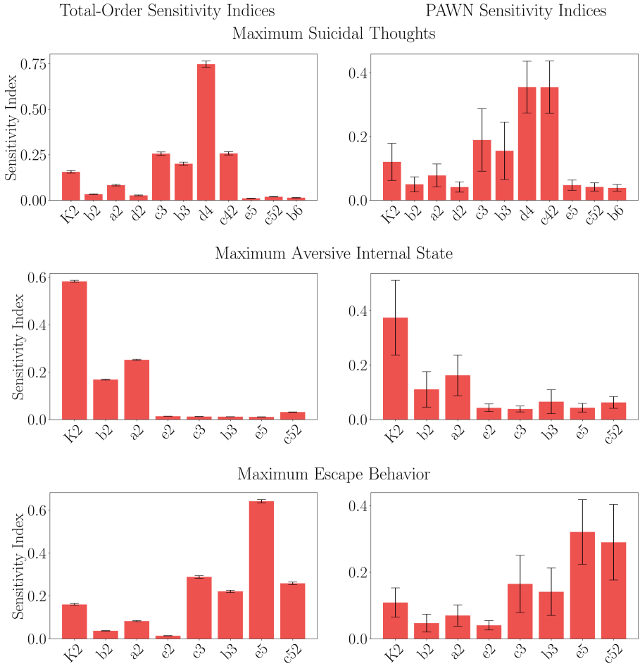
Fig. 5. Total-order Sobolj sensitivity indices (left) and PAWN sensitivity indices (right) for the maximum of the specified model output. Error for Sobolj indices is measured as a 95% confidence interval and the coefficient of variation as error for PAWN indices. Only parameters with an index greater than 0.01 are visualized for ease of reading. Sobolj sensitivity indices were calculated with 2^{17} samples, compared with PAWN sensitivity indices calculated with 2^{14} samples.
