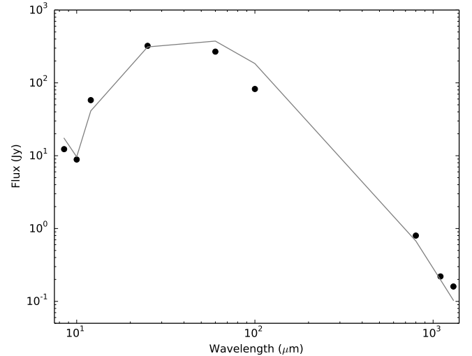
Fig. 4. Spectral energy distribution of IRAS 17150–3224 in black dots. The 8.5 and 10.0 \mu\text{m} points are from Ueta et al. (2000), the 12 , 25 , 60 , and 100 \mu\text{m} points from IRAS, the 800.0 and 1100.0 \mu\text{m} points from Hu et al. (1993) and the 1.3 \text{ mm} from Guertler et al. (1996). In grey is our model based on the parameters of Meixner et al. (2002).
