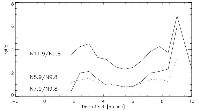
FIG. 4.—Intensity ratio of the PAH bands with respect to N9.8 (pseudo-continuum) along declination through the source center (R.A. offset = 5''6). The data are smoothed to a 0''4 grid. The approximate error levels are about 0.8–1.0.
