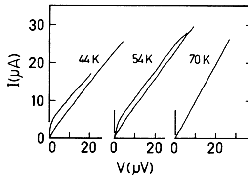
FIG. 4. The extremes of the I - V characteristics (obtained by varying B ) at several different temperatures. Between 50 and 66 K there is no zero-voltage part, but the voltage at constant current still oscillates with the magnetic field. Above 66 K the I - V curves are straight lines and V is independent of the magnetic field within our present experimental accuracy.
