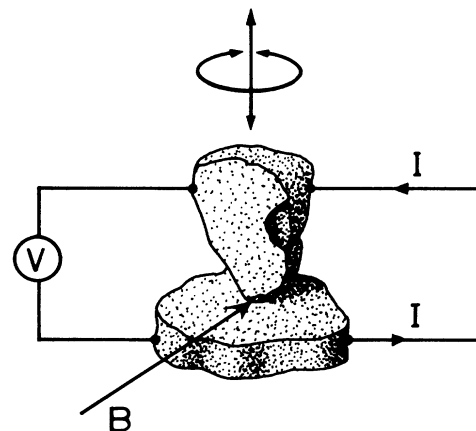
FIG. 1. Schematic diagram of the experimental setup. A little block (sizes on the order of a few mm) of tin or Y-Ba-Cu-O can be lifted up and down, and rotated around a vertical axis. It is pressed against a plate of Y-Ba-Cu-O. The I - V relationship is determined with a four-terminal method. A magnetic field is applied in the horizontal direction.
