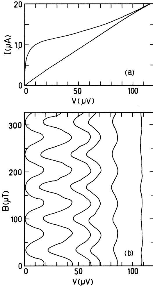
FIG. 3. The I - V - B dependence of the Y-Ba-Cu-O-Y-Ba-Cu-O contact at 4.2 K. (a) I - V characteristics. The set of two curves represents the two extremes between which the characteristics oscillate when B is varied. (b) V - B characteristics for several different currents. The periodicity is the result of a double point contact in the junction between the two pieces of Y-Ba-Cu-O.
