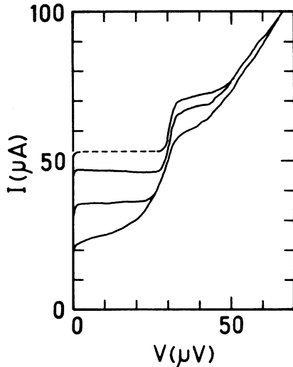
FIG. 2. I - V characteristics of the Sn-Y-Ba-Cu-O contact at 3.65 K. The different curves correspond to different magnetic field values.
