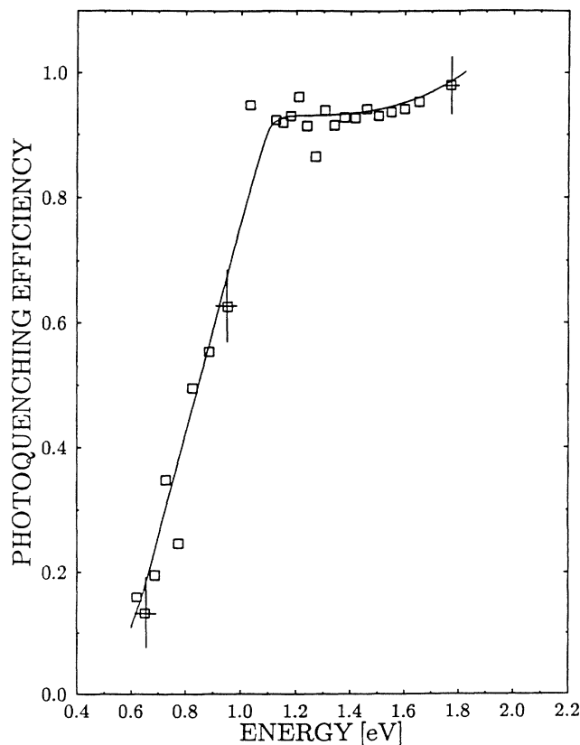
FIG. 2. Spectral dependence of the g = 1.94 ESR signal photoquenching observed for the x = 0.41 \text{Al}_x\text{Ga}_{1-x}\text{As} LPEE epilayer under illumination. The sequence of steps of the experiment is described in the text. 1 stands for total photoquenching of the signal.
