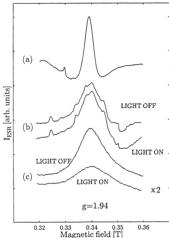
FIG. 1. Electron-spin-resonance spectra of LPE-grown x = 0.42 (a) and x = 0.5 (b) \text{Al}_x\text{Ga}_{1-x}\text{As} layers. The spectra shown in (b) were measured before and after the illumination. The ESR spectrum shown in (c) was measured for x = 0.41 LPEE layer after removing the GaAs substrate. The ESR signal shown was observed for sample cooled down to 4 K temperature in total darkness before and after 120 s of white-light illumination.
