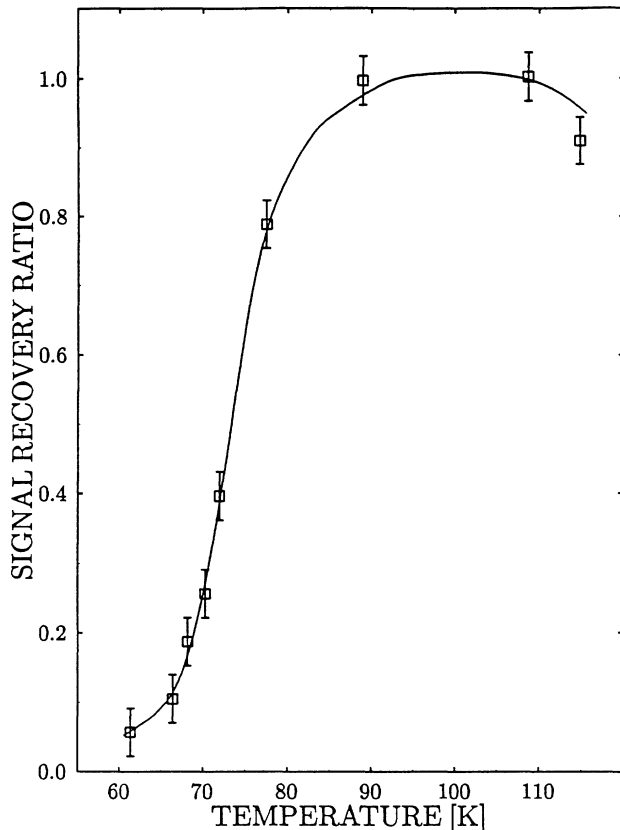
FIG. 3. Temperature dependence of the ESR signal recovery measured for the x = 0.41 \text{Al}_x\text{Ga}_{1-x}\text{As} LPEE epilayer. The sequence of steps of the experiment is described in the text.
