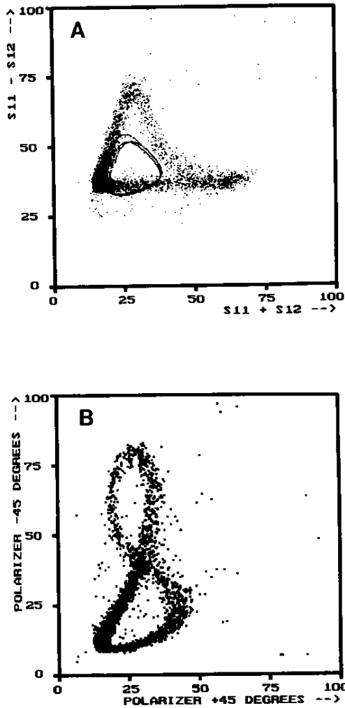
FIG. 3. A: Scatter plot of S_{11}-S_{12} vs. S_{11}+S_{12} signals from 7.040 \mu\text{m} beads measured with the setup using an incident polarization at +45^\circ and a vertical and horizontal, respectively, perpendicular detected polarization at 632.8 nm. The smooth line was calculated assuming a Gaussian size distribution (bead size range: 6.84 \mu\text{m} to 7.24 \mu\text{m} , wavelength is 632.8 nm). B: Scatter plot of 7.040 \mu\text{m} beads when the incident polarization is right circular and the perpendicular detected polarization is -45^\circ and +45^\circ (wavelength is 632.8 nm). This corresponds to S_{11} - 0.62 \cdot S_{33} - 0.78 \cdot S_{34} vs. S_{11} + 0.62 \cdot S_{33} + 0.78 \cdot S_{34} .
