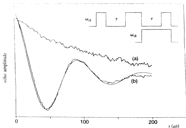
FIG. 2. Optically detected Hahn-echo decay (in arbitrary units) of the |D| - |E| zero-field transition (at 1870 MHz) of the F_2^{2+} center in CaO in the photoexcited ^3B_1 state at 1.3 K (a) without pumping the |D| + |E| transition; (b) with the simultaneous pumping at \tau < t < 2\tau of the |D| + |E| transition (at 2230 MHz); see also insert. Drawn line is simulated Autler-Townes modulation.
