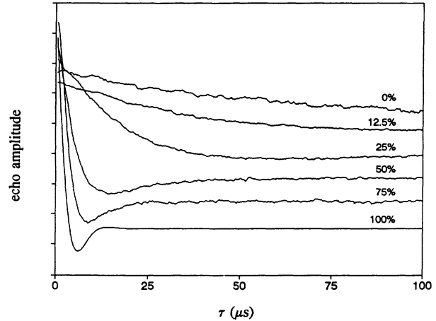
FIG. 3. Autler-Townes modulation of the |D\rangle - |E\rangle zero-field transition (at 1870 MHz) of the F_2^{2+} center in CaO in the photoexcited {}^3B_1 state for a series of power levels of the pumped |D\rangle + |E\rangle transition (at 2230 MHz).
