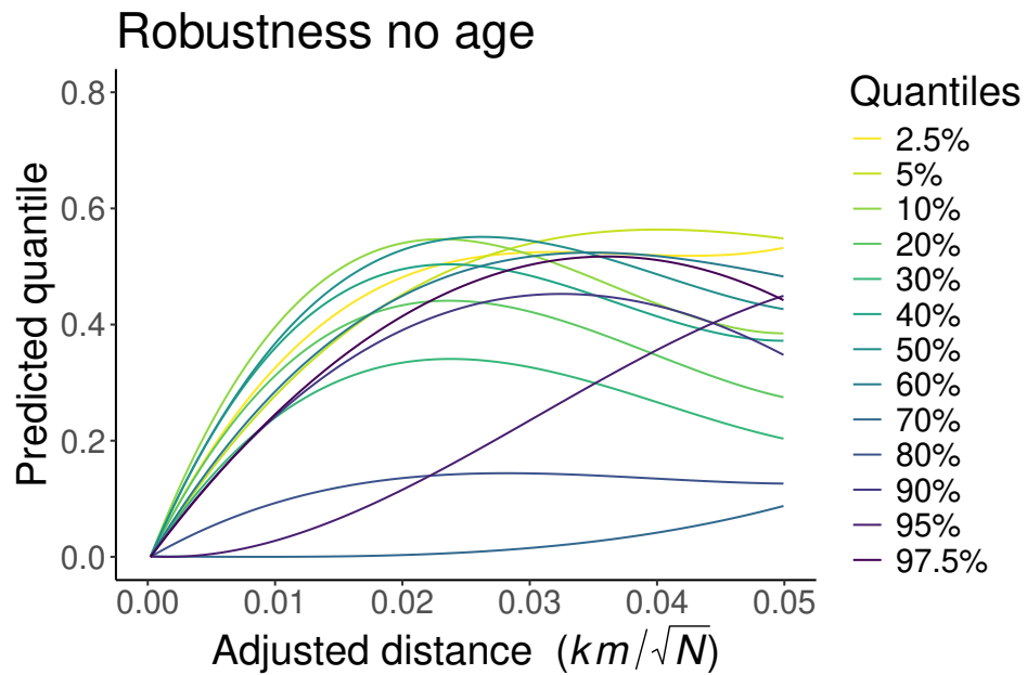
Supplementary Figure S5: Results when the analysis is run without controlling for age.
