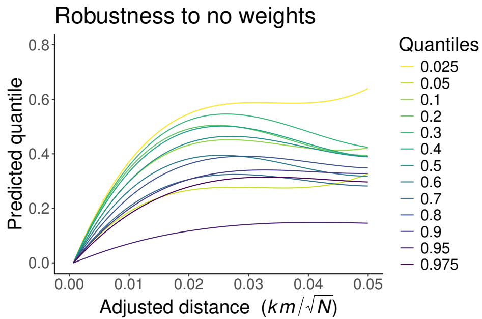
Supplementary Figure S6: Results when the analysis is run without participant weights.
