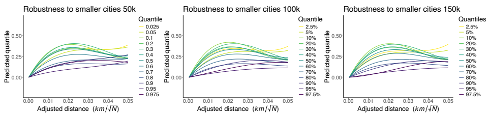
Supplementary Figure S3: Results when including city centers of cities with more than 50k, 100k, and 150k inhabitants. The main analysis uses a minimum criterion of 200k.
