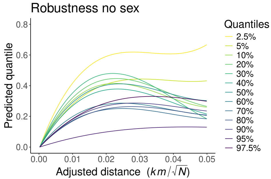
Supplementary Figure S4: Results when the analysis is run without controlling for sex.
