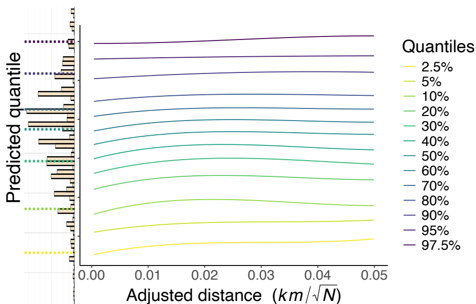
Supplementary Figure S1: Predicted 2.5%, 50%, and 97.5% quantiles as a function of adjusted distance.
