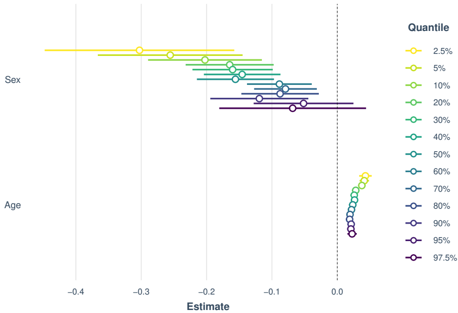
Supplementary Figure S2: Estimated coefficients for 13 quantiles with 95% confidence intervals. Sex show the linear effect of sex on the quantiles, while age shows the linear effect of age. A negative effect of sex means that quantiles are lower for men, while the positive effect of age shows that quantiles increase with age.
