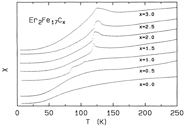
FIG. 3. Ac susceptibility vs temperature for \text{Er}_2\text{Fe}_{17}\text{C}_x compounds.
