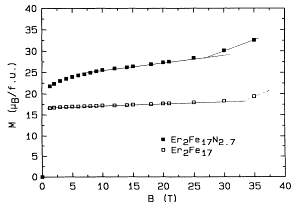
FIG. 9. Magnetic isotherms at 4.2 K for free-powder samples of \text{Er}_2\text{Fe}_{17}\text{N}_{2.7} and \text{Er}_2\text{Fe}_{17} . The lines are guides to the eye.
