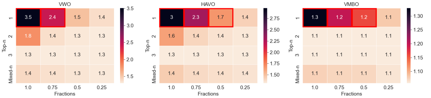
Figure 1: Average rank of RM-HAL matches when agents apply the first-order heuristic strategy for varying values of n and f . Scenarios where RM-HAL has a worse average rank than RSD are highlighted in red.
