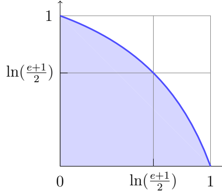
Figure 4.1: An illustration of the region R = \{(a, b) \in [0, 1]^2 : f(a) + f(b) \leq 1\} . The symmetric point at the boundary of the region has both coordinates \ln((e + 1)/2) \approx 0.62 . When an online node w arrives, a threshold respecting algorithm ensures that the fractional matching x satisfies (x(\delta(u)), x(\delta(v))) \in R for every hyperedge h = \{u, v, w\} \in \delta(w) with x_h > 0 at the end of that iteration.
