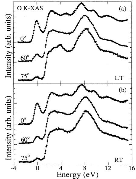
FIG. 1. Normalized O K -edge XAS spectra of the Bi2212 system collected at different angles of incidence with respect to the normal of the sample surface at temperatures below T_c (a) and at room temperature (b). The 0^\circ spectrum corresponds to the normal incidence geometry where the E vector of the plane-polarized synchrotron light is parallel to the sample surface ( ab plane), while the 75^\circ spectrum represents the case where the E vector is nearly parallel to the c axis of the crystal.
