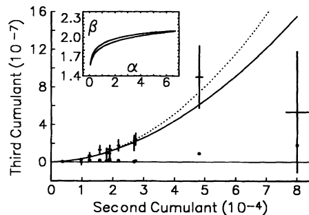
FIG. 4. The third cumulant as a function of the second cumulant of the intensity distribution. Solid line is weighted least squares fit to the data of \langle \langle T_a^3 \rangle \rangle = \alpha \langle \langle T_a^2 \rangle \rangle^\beta . The inset shows the 68% confidence region of the fit parameters \alpha and \beta , yielding \alpha = 0.7_{-0.7}^{+6.0} , \beta = 1.83 \pm 0.26 . Dashed line is theoretical prediction \langle \langle T_a^3 \rangle \rangle = 3.2 \langle \langle T_a^2 \rangle \rangle^2 . Dots show the upper bound of the contribution of the mundane diagram in Fig. 3(b) to the third cumulant.
