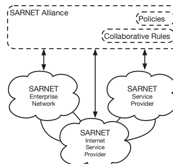
Fig. 2: A SARNET alliance enforces a common set of rules on collaborating networks.
