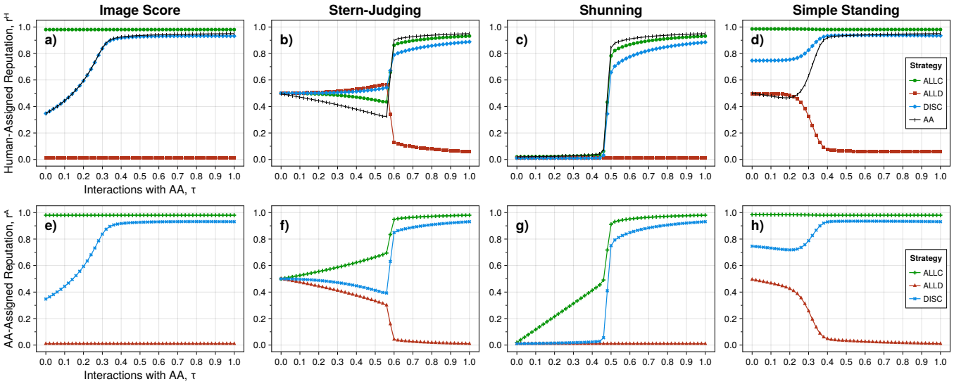
Figure 6: Average reputations, r_s^H, s \in S and r_A^H (top) and r_s^A, s \in S (bottom), at different frequencies of interaction with a DISC AA, when d^A = IS , and varying d^H . Introducing an AA increases the average human and AA-assigned reputation of DISC and/or ALLC relative to ALLD, resulting in more targeted punishments. We follow the same parameters as Figure 2, with b/c = 3 .
