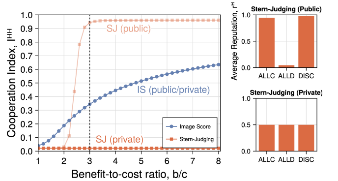
Figure 2: Left: Human cooperation under public and private reputations, I^{H,H} , without artificial agents, for two exemplifying social norms and benefit-to-cost ratios, b/c . Right: The average reputation assigned to each strategy under public (top) and private (bottom) reputations ( b/c = 3 ). While cooperation increases with b/c under public reputation, when reputations are private cooperation remains close to 0 for every norm except IS, which still leads to low ( < 0.65 ) cooperation. This is attributed to lack of distinguishability between strategies, leading to DISCs being unable to punish defectors. Z = 100, e_e = e_a = 0.01, \gamma = 0.01, \beta = 1 .
