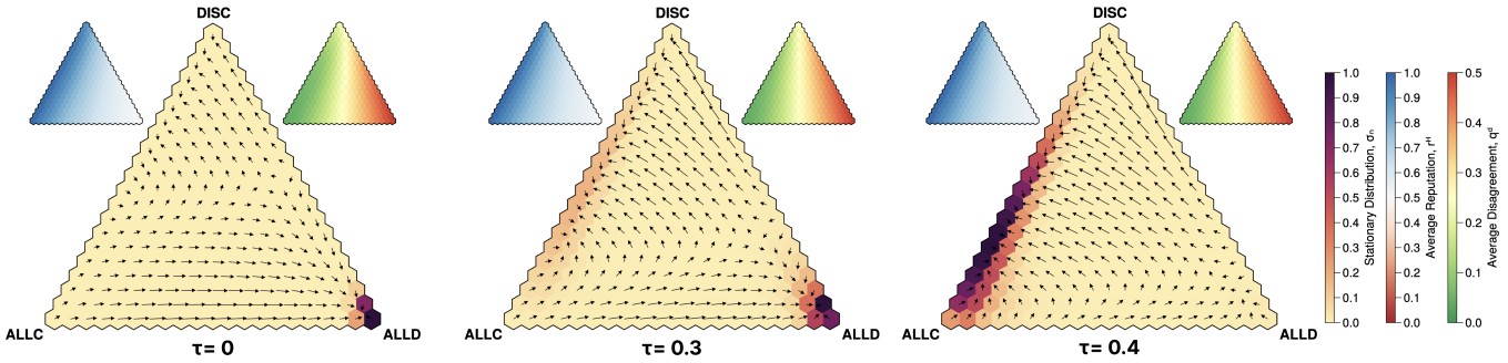
Figure 4: The stationary distribution (rescaled such that the maximum value is 1), gradient of selection, average reputation and average disagreement at each strategy state for different frequencies \tau of interaction with a DISC AA, when d^A = \text{IS} and d^H = \text{SS} . The population transitions from an ALLD state, with high reputation disagreement, to states where ALLC and DISC co-exit and every agent accrues the same (good) reputation, resulting in higher cooperation. We follow the same parameters as Figure 2.
