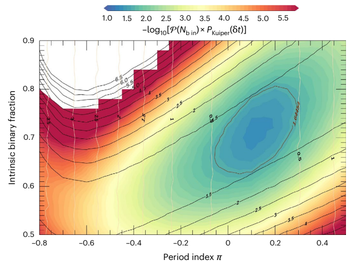
Fig. 3 | Two-dimensional map combining the binomial probability \mathcal{P} and Kuiper statistics P_{\text{Kuiper}} of simulated populations to reproduce the observable multiplicity properties of our BLOeM sample. The equi-probability contours of the two-sided Kuiper statistics (vertical lines) and the probability to detect the same number of binaries as we do (diagonal lines) are overlaid. The colour scale gives the logarithm of the products of both probabilities. The red contour indicates the half-peak value.
