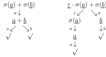
Fig. 2. Graphical two-phase presentation of two processes.
