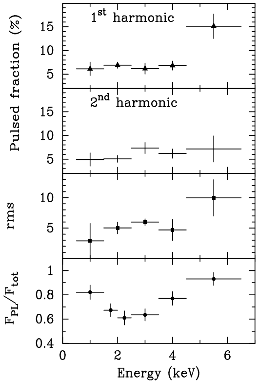
Fig. 5. Pulsed fraction of the first two harmonics of 4U 0142+61 as a function of the energy for observation A (upper two panels), together with the rms and the power-law to total flux ratio (lower two panels). See text for details.
