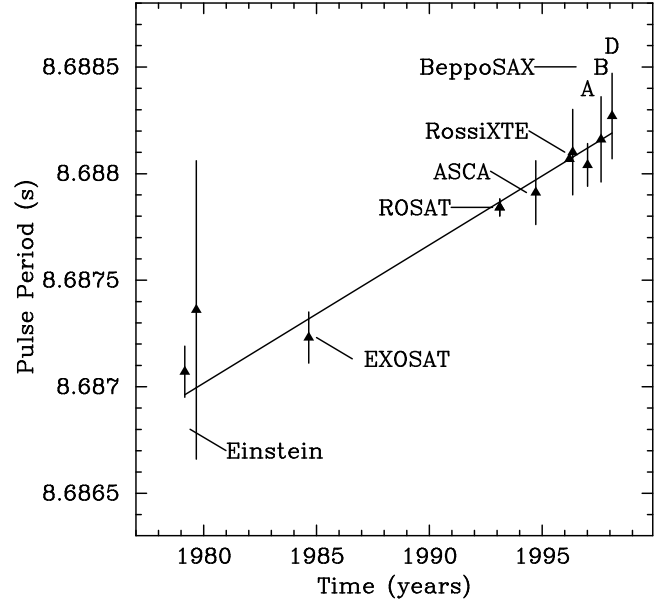
Fig. 4. Pulse period history of 4U 0142+61 as a function of time. 1\sigma uncertainties have been used.
