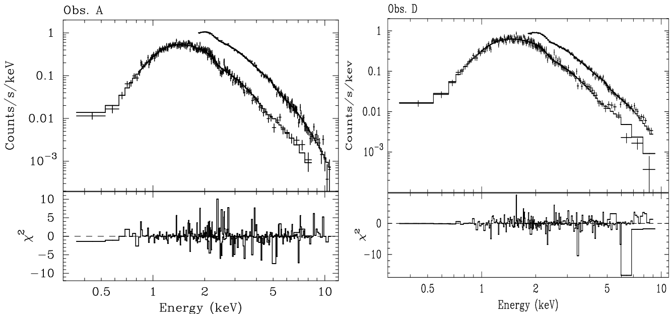
Fig. 1. LECS and MECS energy spectra of 4U 0142+61 during observation A (left panel) and D (right panel). The best fit spectral model (PL+BB; see text for details) is also shown together with the \chi^2 residuals.
