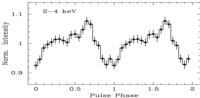
Fig. 6. The 4U 0142+61 RXTE 2–4 keV light curve folded to the best fit period ( P=8.6881 s).
