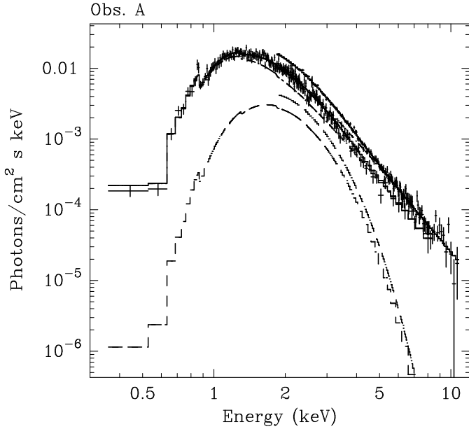
Fig. 2. 4U 0142+61 LECS and MECS unfolded spectrum for observation A. The power-law and blackbody components are shown (dotted and stepped lines).
