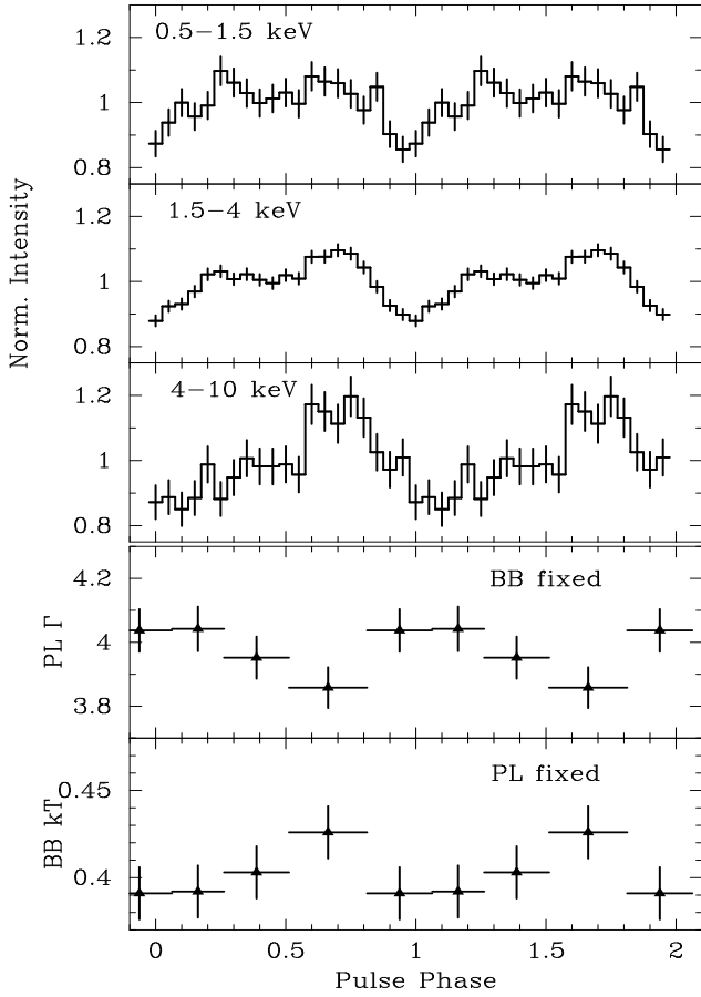
Fig. 3. The 4U 0142+61 MECS light curves for obs. A (first three panels) folded to the best period ( P=8.68804 s) in the 0.5–1.5 keV, 1.5–4 keV and 4–10 keV energy bands. Zero phase was (arbitrarily) chosen to correspond to the minimum in the 1.5–4 keV folded light curve. The results of the pulse phase spectroscopy of obs. A (last two panels) are also reported for two spectral parameters. For clarity two pulse cycles are shown.
