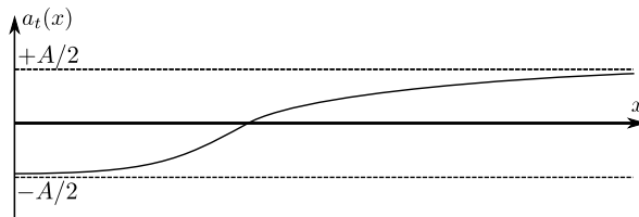
Figure 3: Plot of a schematic form of the potential a_t(x) . We assume that A < 2m .
