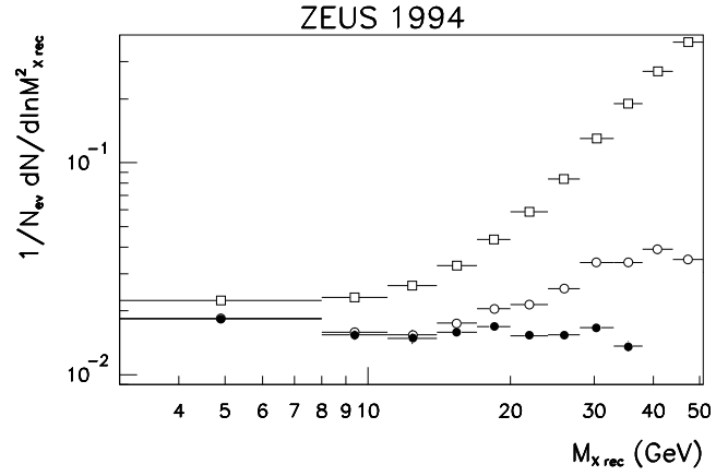
Fig. 4. Uncorrected spectrum of reconstructed hadronic mass in photoproduction events at W \approx 200 GeV before (squares) and after (open circles) imposing the requirement of no hits in the PRT. The latter spectrum was subject to subtraction of the nondiffractive contamination resulting in the uncorrected distribution attributed to diffractive processes (solid points)
