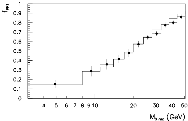
Fig. 5. The fraction of events with a PRT hit as function of the reconstructed mass M_{X\text{ rec}} for data (solid points) and for MC (line)
