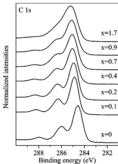
FIG. 5. C 1s core-level spectra of CuPc as a function of K intercalation ( K_x CuPc).
