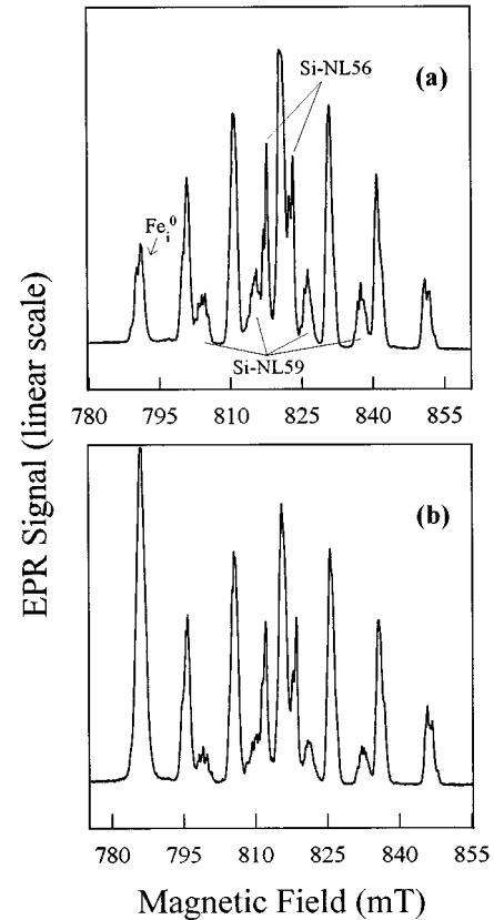
FIG. 1. EPR spectra observed with magnetic field in the (0\bar{1}1) plane at an angle of 40^\circ away from the [100] crystal direction for a sample doped with (a) 107 Ag (microwave frequency \nu = 22.9224 GHz); (b) 109 Ag ( \nu = 22.7818 GHz) silver isotopes. Temperature T = 4.2 K.
