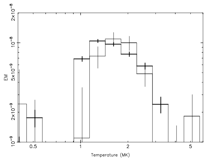
Fig. 3. EM ( n_e n_{\text{H}} V in 10^{64} \text{ m}^{-3} ) for RGS and LETGS (thick), using the regularisation algorithm. The relative abundances given in Table 4 have been applied.
