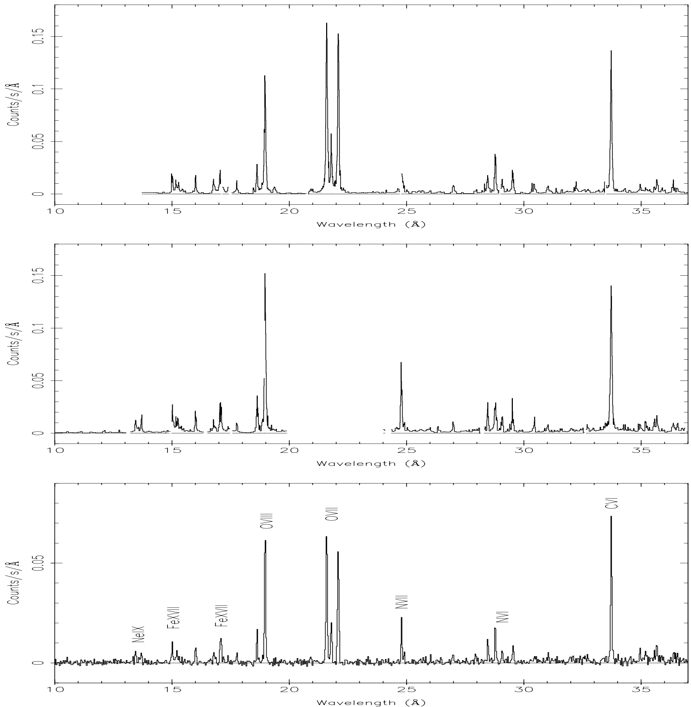
Fig. 1. From top to bottom the spectra of Procyon observed by RGS1, RGS2 and LETGS in the wavelength region from 10 to 37 Å.
