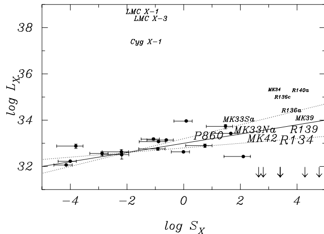
FIG. 5.—X-ray luminosity as a function of S_X (eq. [1]). The bullets give the location of the binaries listed by Chlebowski & Garmany (1991). The Chandra X-ray sources from Table 2 are identified by their optical counterpart; the size of their names are proportional to the 1 \sigma errors. The solid line gives a least-squares fit to the bullets, which represent the sources of Table 3. The dotted lines represent the uncertainty interval of the fit. For comparison, we plot the location of three known high-mass X-ray binaries with a black hole (see discussion). The values of S_X (eq. [1]) for the five downward-pointed arrows represent the stars (from left to right) R136b, Mk 37Wb, Mk 35, Mk 30, and Mk 49, which we did not detect in X-rays.
