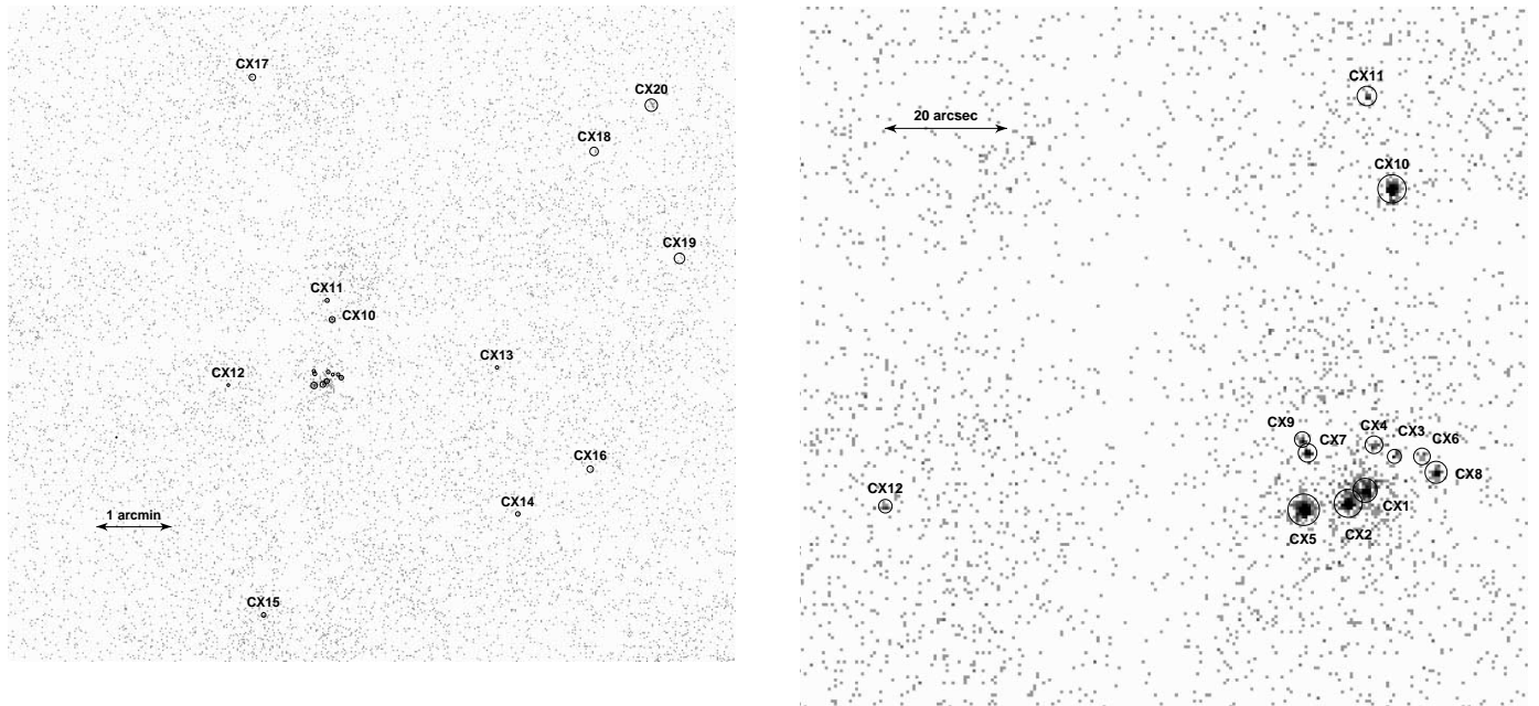
FIG. 1.—X-ray image of the star cluster R136 in the 30 Doradus region. ( left ) 11' \times 11' view; ( right ) close-up of the cluster. The sources are identified in Table 1.
