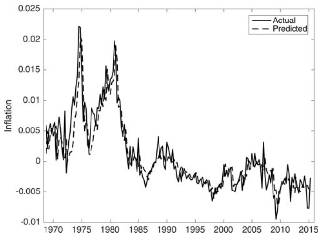
Figure 1. Actual versus predicted inflation.
