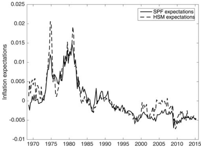
Figure 3. Inflation expectations: SPF data and HSM prediction.
