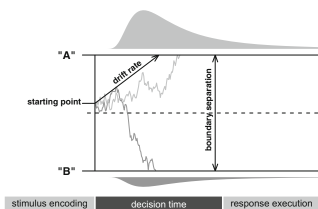
Fig. 1 Graphical illustration of the diffusion model
