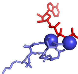
Figure 2.5: Biological function of the third prebiotic peptide candidate. The figure is drawn using Pymol ( http://pymol.sourceforge.net ). DAKVGDGD motif: PDB entry 1un9 A380-A387 bound to two Mg^{2+} ions (blue) and interacting with an ATP molecule (red).
