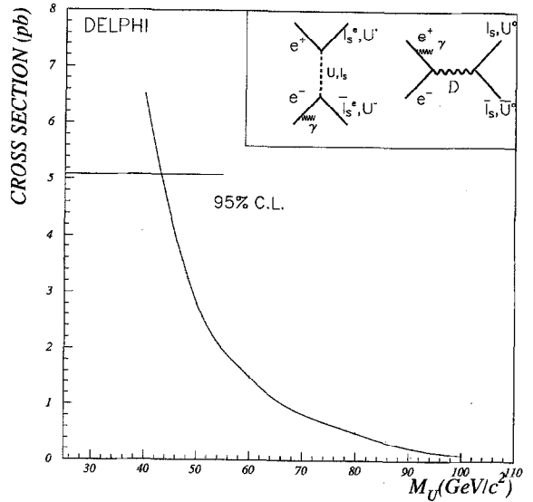
Fig. 4. Limit at 95% C.L. for the mass of the W -type U boson. The curve shows the predicted cross section as a function of M_U according to [10]. The insert shows two examples of the Feynman graphs contributing to the calculated cross-sections.
