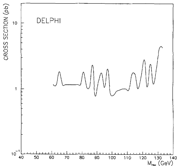
Fig. 5. Upper limit at 95% C.L. for the cross-section of \gamma X final state as a function of the mass of X.
