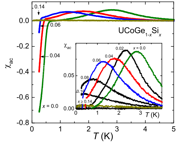
FIG. 2. (Color online) Temperature variation of the ac susceptibility (SI units) of \text{UCoGe}_{1-x}\text{Si}_x alloys for x=0.00, 0.04, 0.06 , and 0.14 . The inset shows \chi_{ac} around the ferromagnetic transition for 0.00 \leq x \leq 0.20 . The data for x=0.20 fall on the horizontal axis.
