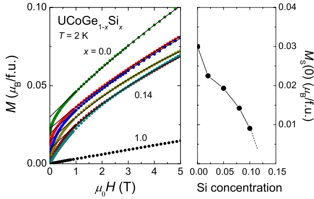
FIG. 1. (Color online) Left panel: magnetization as a function of field for \text{UCoGe}_{1-x}\text{Si}_x alloys at T=2 K. Si concentrations are (from top to bottom) x=0, 0.02, 0.05, 0.08, 0.10, 0.14 , and 1.0 . The solid lines represent fits to Eq. (1) for x \leq 0.10 . Right panel: spontaneous magnetization M_s(0) as a function of Si content.
