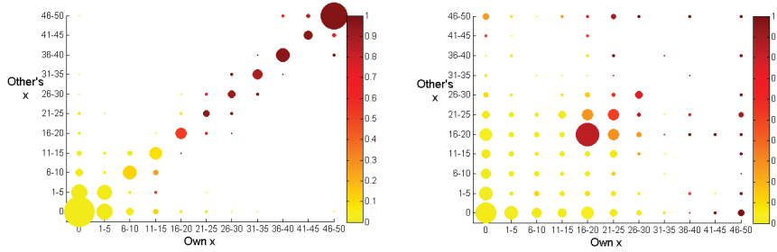
Figure 4: Cooperation probability for a given punishment level pair in the Gradual (left panel) and in the Leap treatments (right panel)
