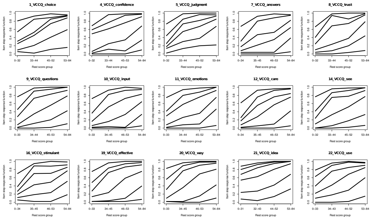
Figure 4.2: ISRFs for the 15-item VCCQ in Study 2 ( N=228 )
