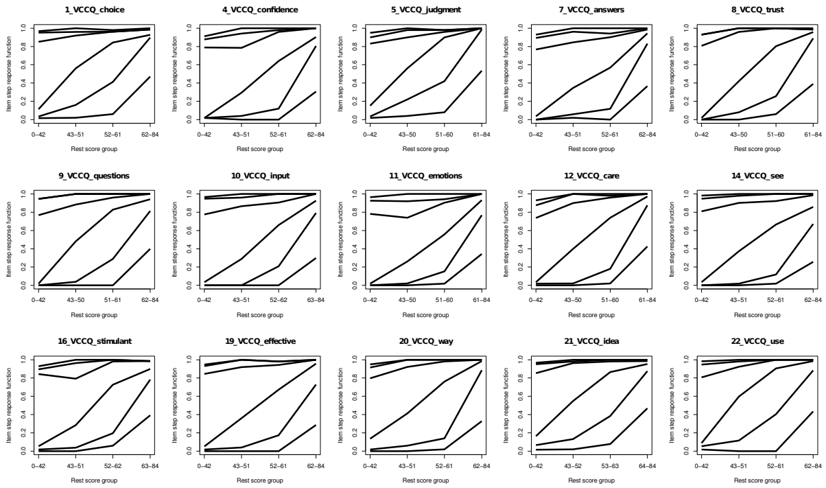
Figure 4.1: ISRFs for the 15-item VCCQ in Study 1 ( N=230 )
