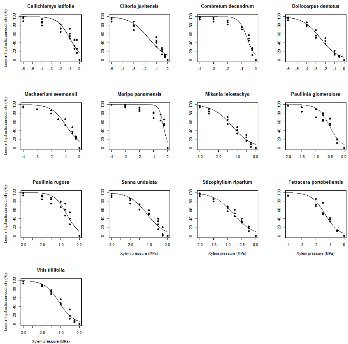
Figure S1: Vulnerability curves showing the loss in hydraulic conductivity with increasing xylem pressure for all liana species of the Soberania forest site.
