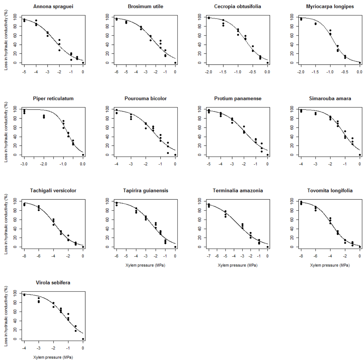
Figure S1: Vulnerability curves showing the loss in hydraulic conductivity with increasing xylem pressure for all tree species of the San Lorenzo forest site.
