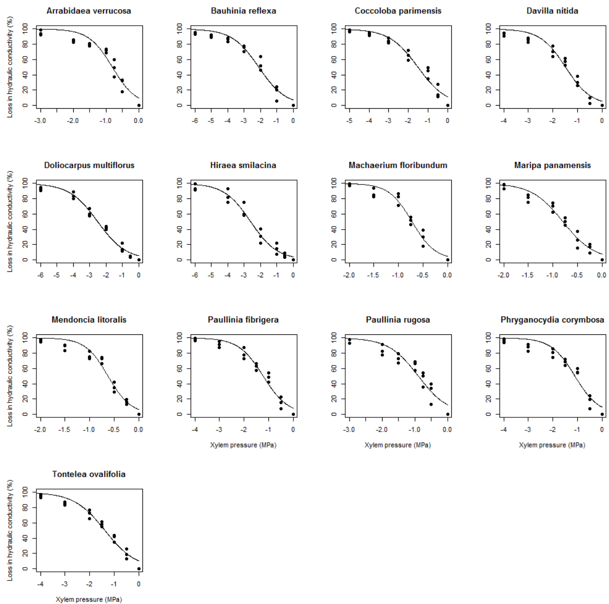
Figure S1: Vulnerability curves showing the loss in hydraulic conductivity with increasing xylem pressure for all liana species of the San Lorenzo forest site.
