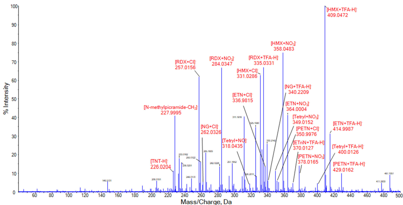
Figure 8. SAWN-MS spectrum of a mixture of PETN, ETN, NG, RDX, HMX, TNT, and tetryl, analyzed in negative ionization mode. Concentration of 1 \mu\text{g/mL} in \text{MeOH} + 0.1 \text{ v\% } \text{CHCl}_3 for each compound. Peaks labeled in red were identified as analyte related (adduct) ions
