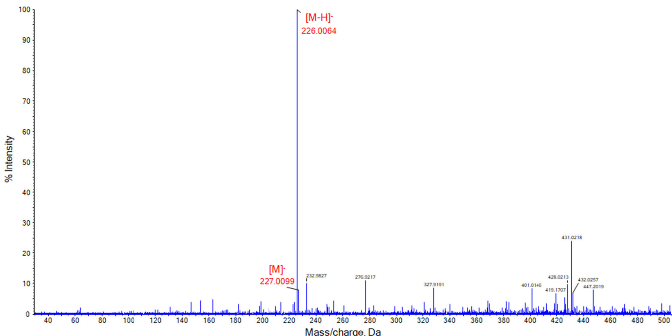
Figure 6. SAWN-MS spectrum of a 1 µg/mL TNT in MeOH, analyzed in negative ionization mode. Peaks labeled in red were identified as TNT-related ions
