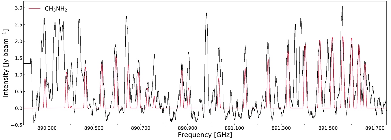
Fig. C.1. \text{CH}_3\text{NH}_2 transitions detected towards NGC 6334I in the range 890.2 to 891.7 GHz (ALMA Band 10). The red line represents the synthetic spectrum of \text{CH}_3\text{NH}_2 assuming a column density of 2 \times 10^{17} \text{ cm}^{-2} , an excitation temperature of 100 K and a FWHM line width of 3.2 \text{ km s}^{-1} , in a 00''.26 \times 0''.26 beam (equivalent to the angular resolution of the data). The abscissa is the rest frequency with respect to the radial velocity towards the region ( -7 \text{ km s}^{-1} ). The data are shown in black.
